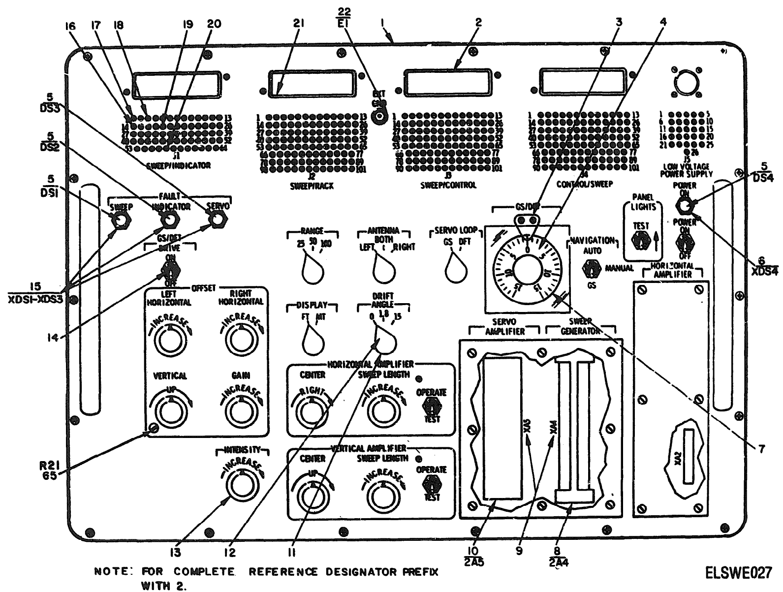
Figure 22. Panel, Test Electrical (Sheet 1 of 3).
