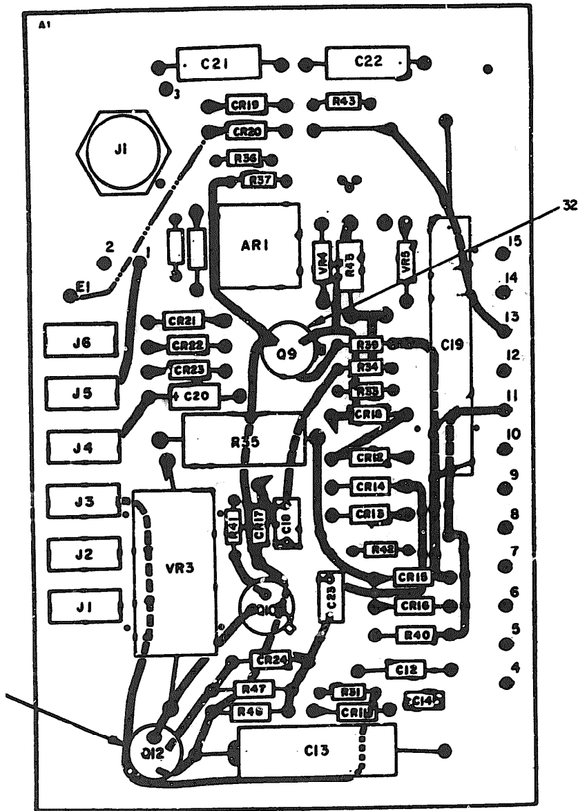
Figure 19. Circuit Card Assembly 1A2A6A1 (Sheet 1 of 2).
