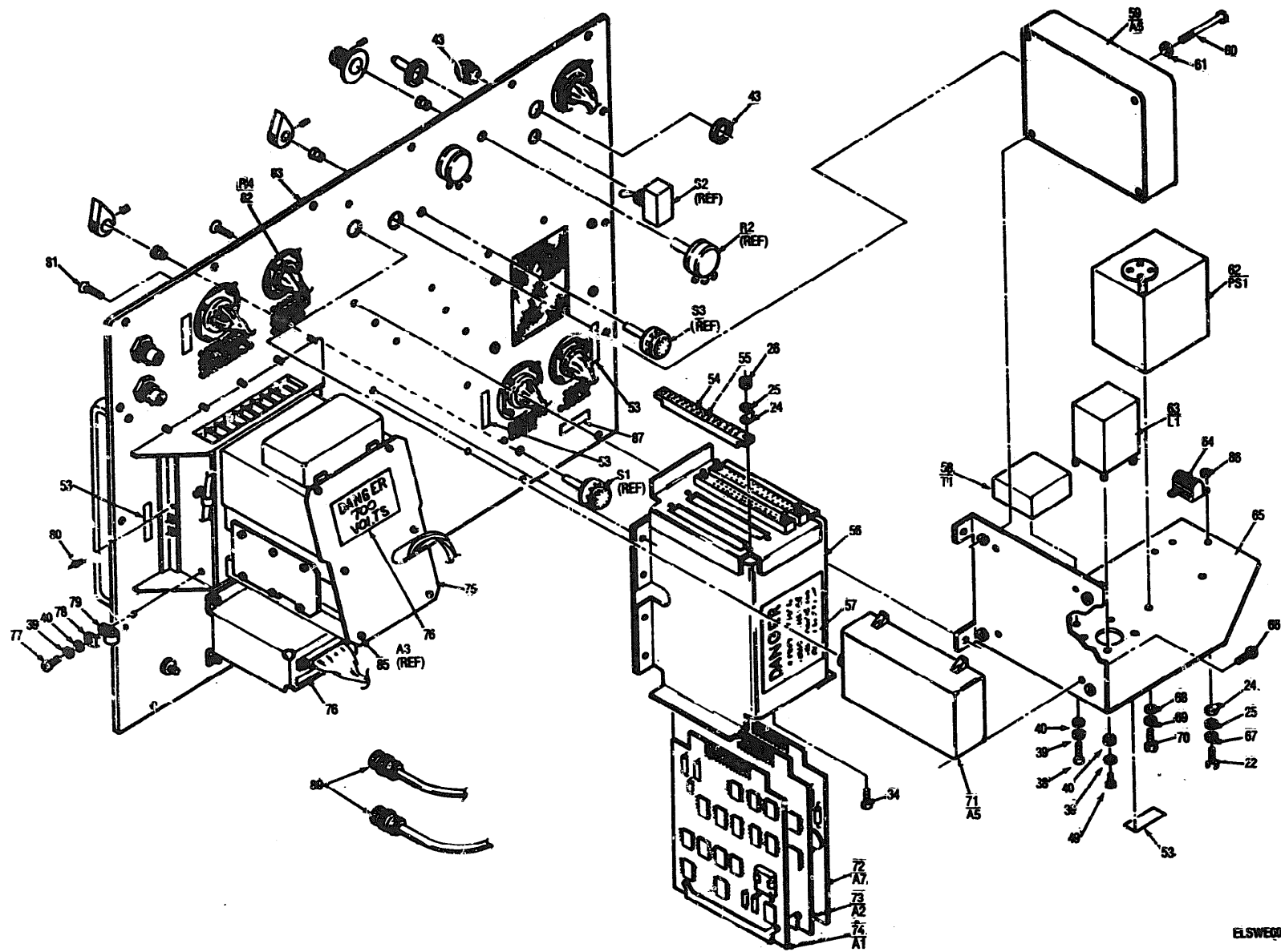
Figure 3. Electrical Test Panel 1A1 (Sheet 3 of 3).
