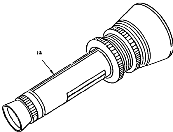
Figure 39. Test Set Subassembly MX-99B4/APS-94D (Sheet 2 of 3).
