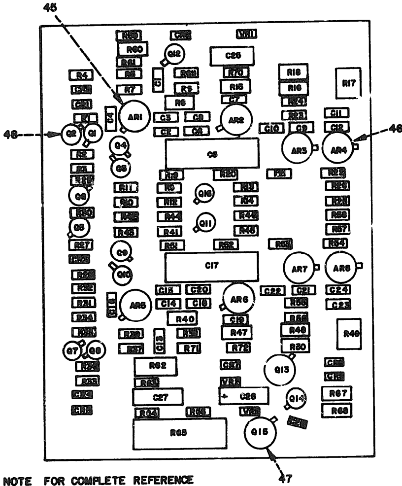
Figure 32. Circuit Card Assembly 2A5A3 (Sheet 1 of 2)
