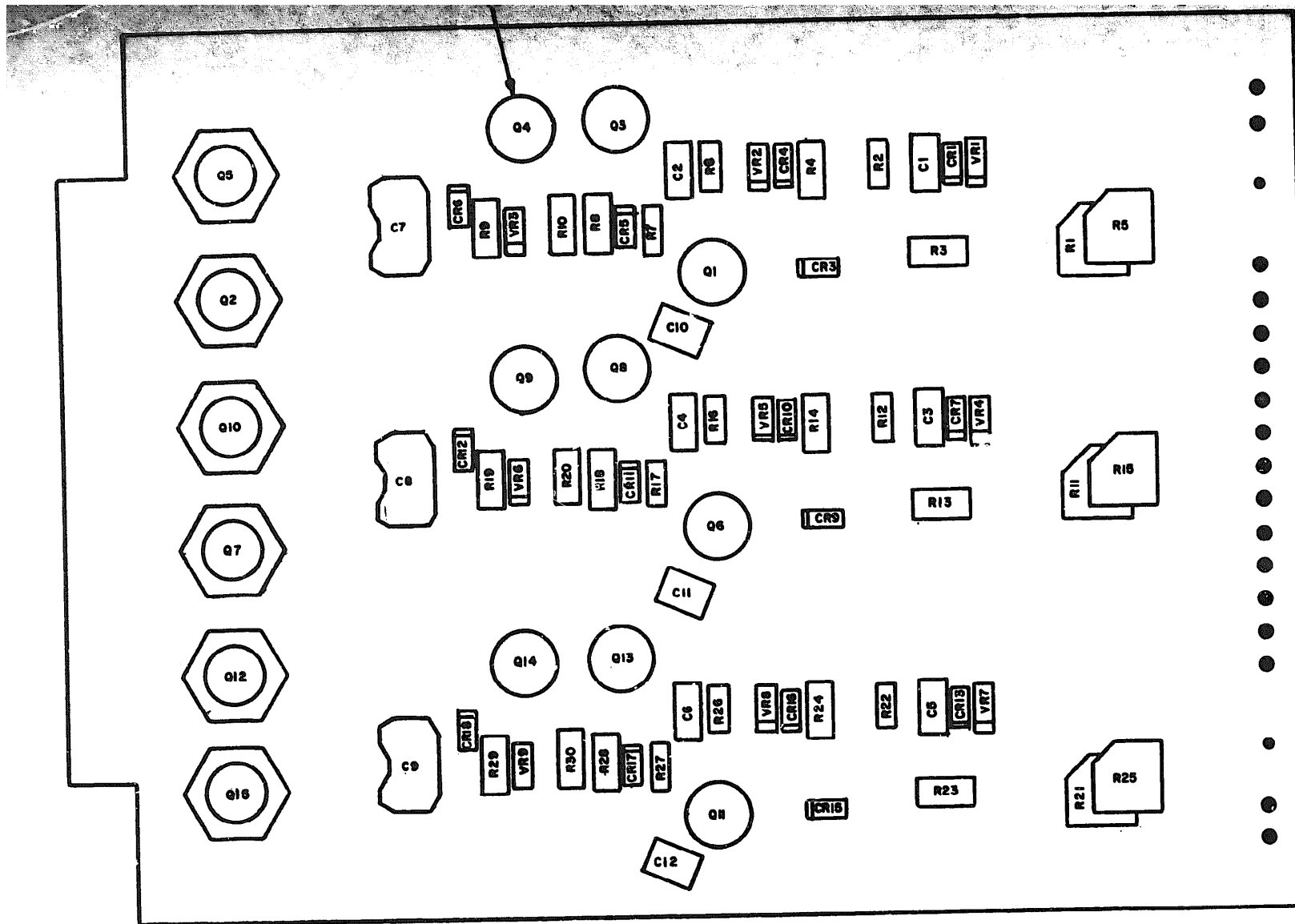
Figure 17. Overvoltage Protector Module 1A2A5 (Sheet 1 of 2).
