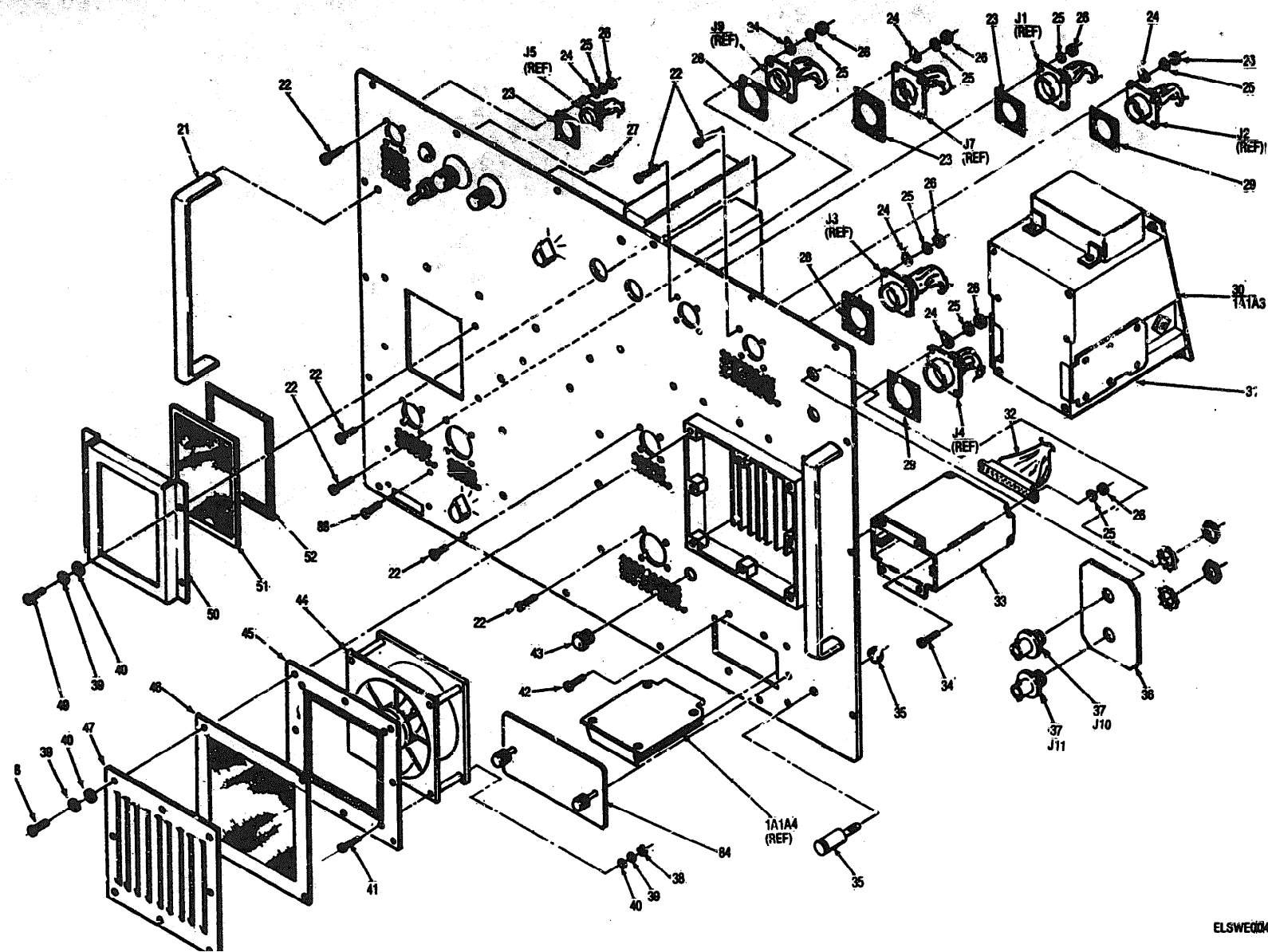
Figure 3. Electrical Test Panel 1A1 (Sheet 2 of 3).
