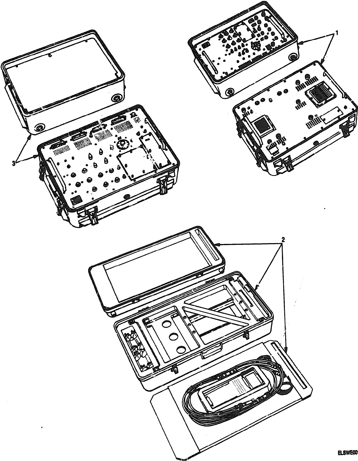
Figure 1. Test Set Group, Indicator, Radar OQ-63A/APS-94D
