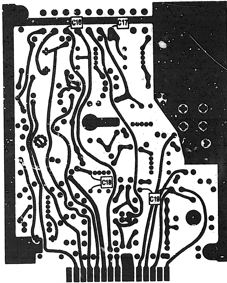
Figure 27. Circuit Card Assembly 2A4A1 (Sheet 2 of 3).
