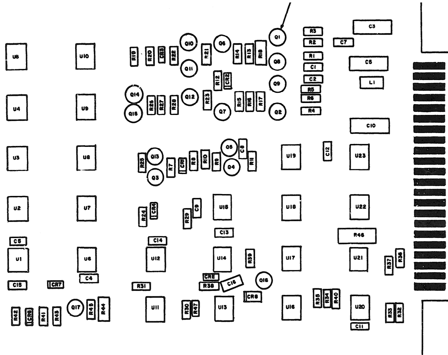
Figure 14. Antenna Counter Module IA2A2 (Sheet 1 of 2).
