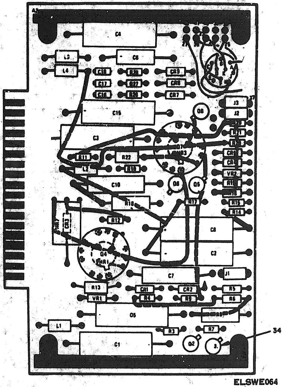
Figure 20. Circuit Card Assembly 1A2A6A2 (Sheet 1 of 2).
