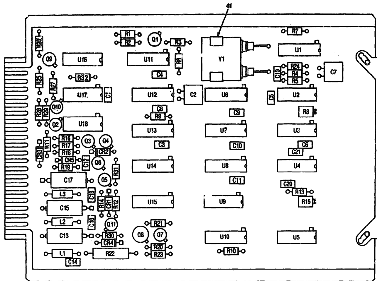
Figure 4. Circuit Card Assembly IAIA1 (ADAS Simulator) (Sheet 1 of 2).
