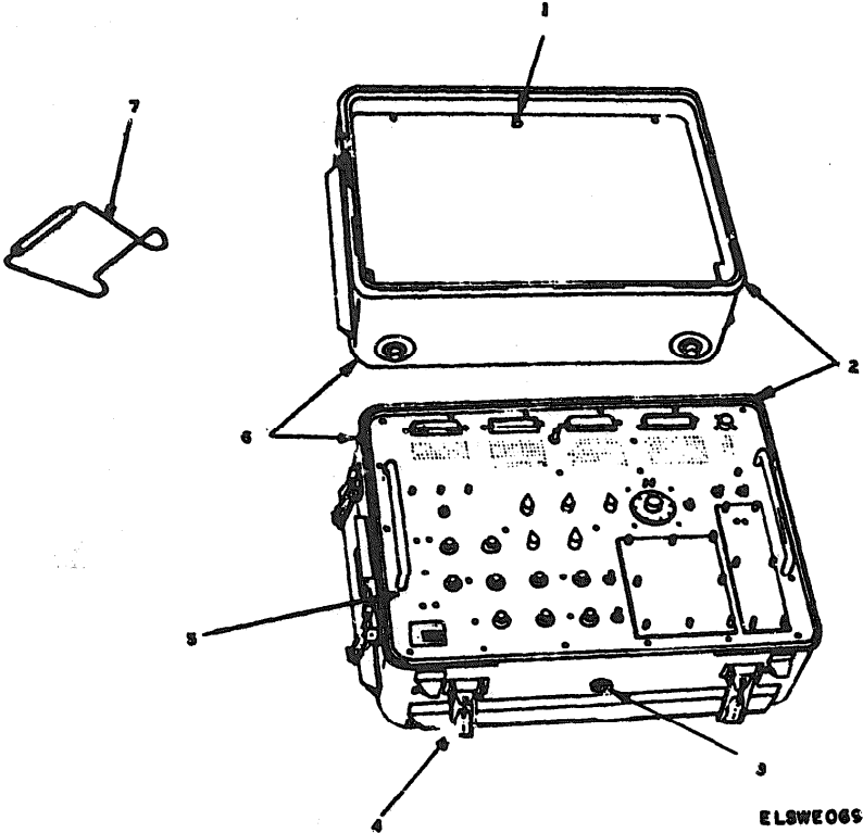
Figure 21A. Test Set Subassembly MX-8639A/APS-94D.
