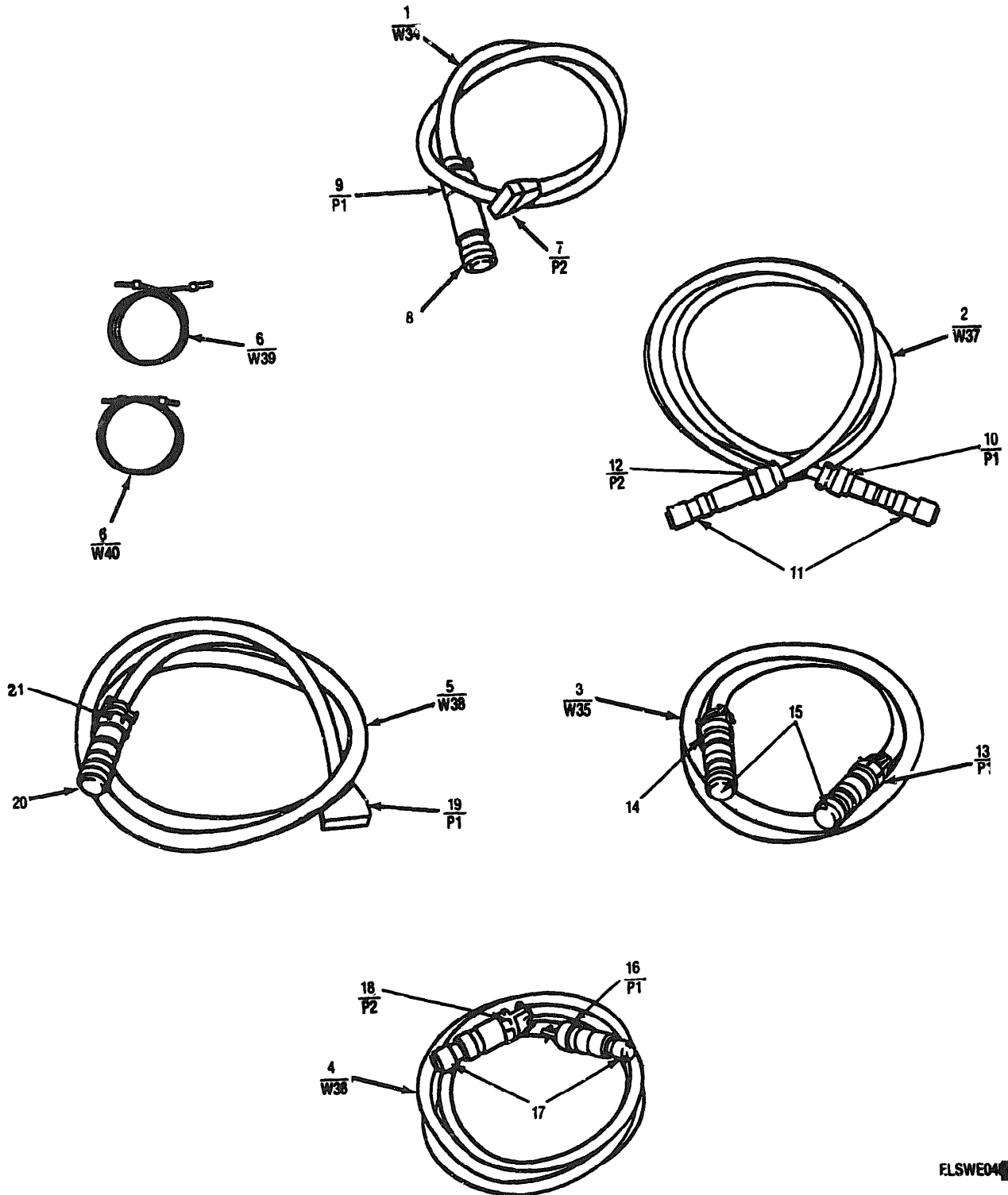
Figure 41. GROUP CABLE ASSEMBLIES
