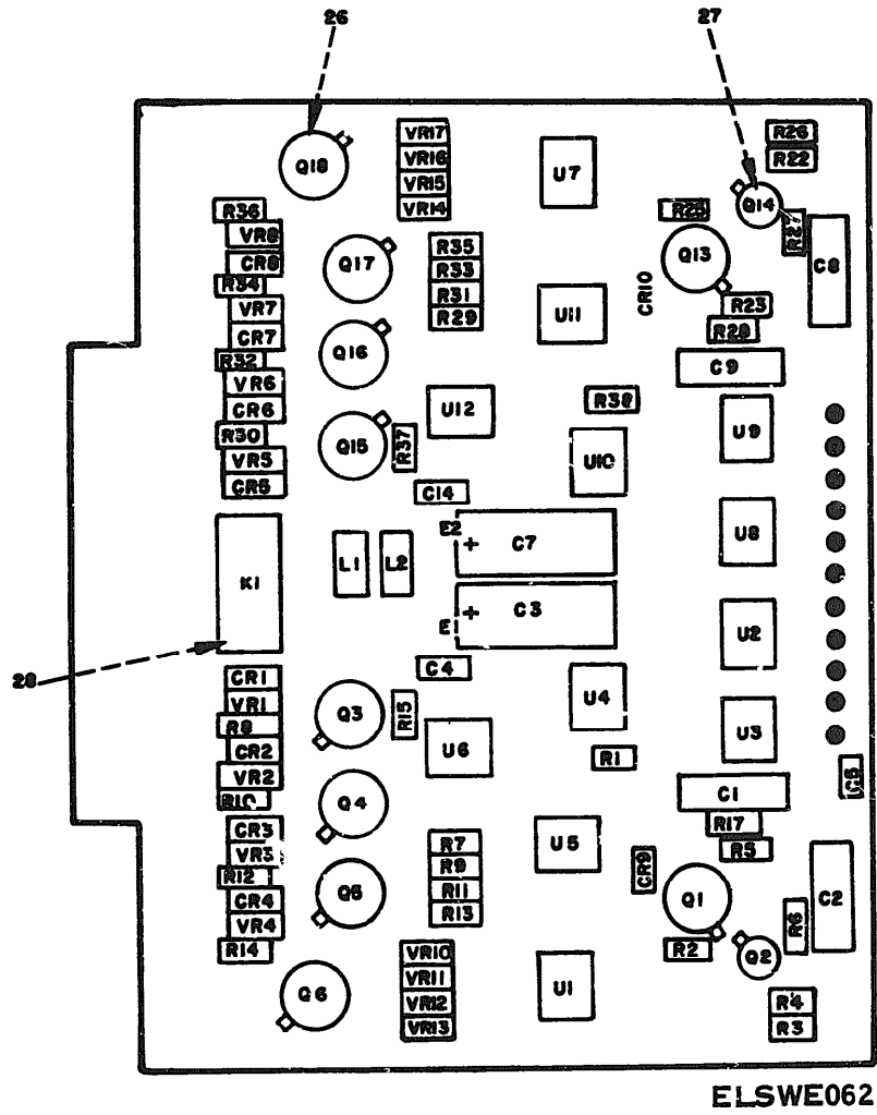
Figure 31. Circuit Card Assembly 2A5A2 (Sheet 1 of 2)
