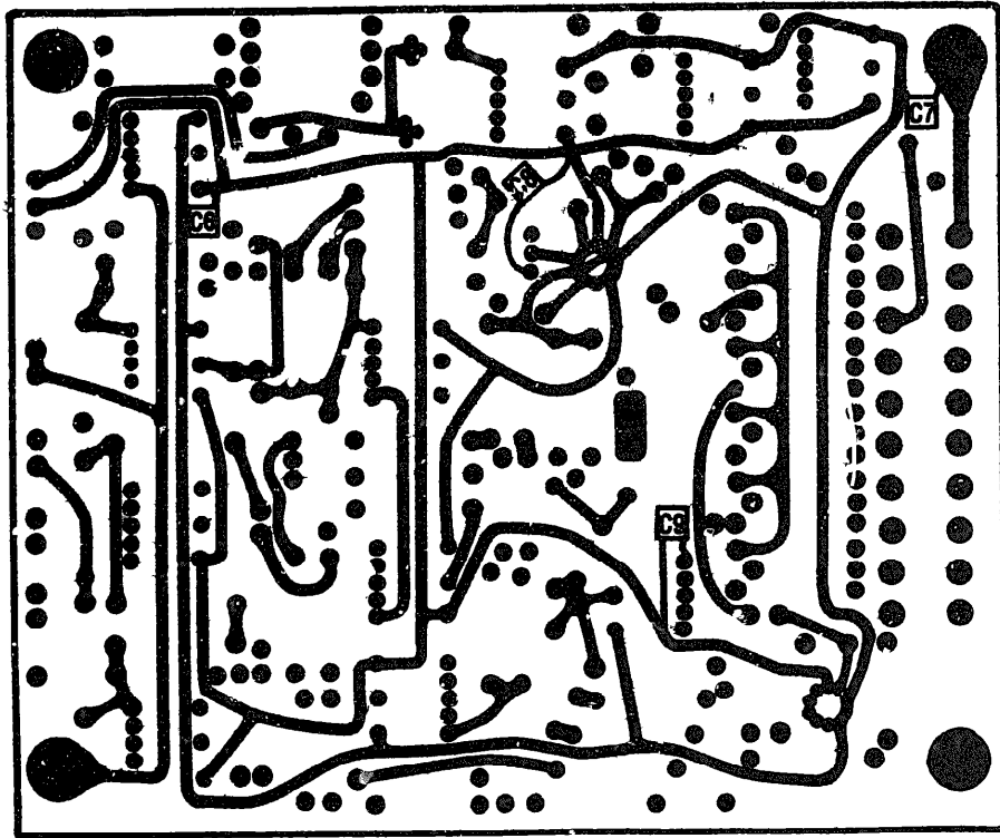
Figure 28. Circuit Card Assembly 2A4A2 (Sheet 2 of 3)
