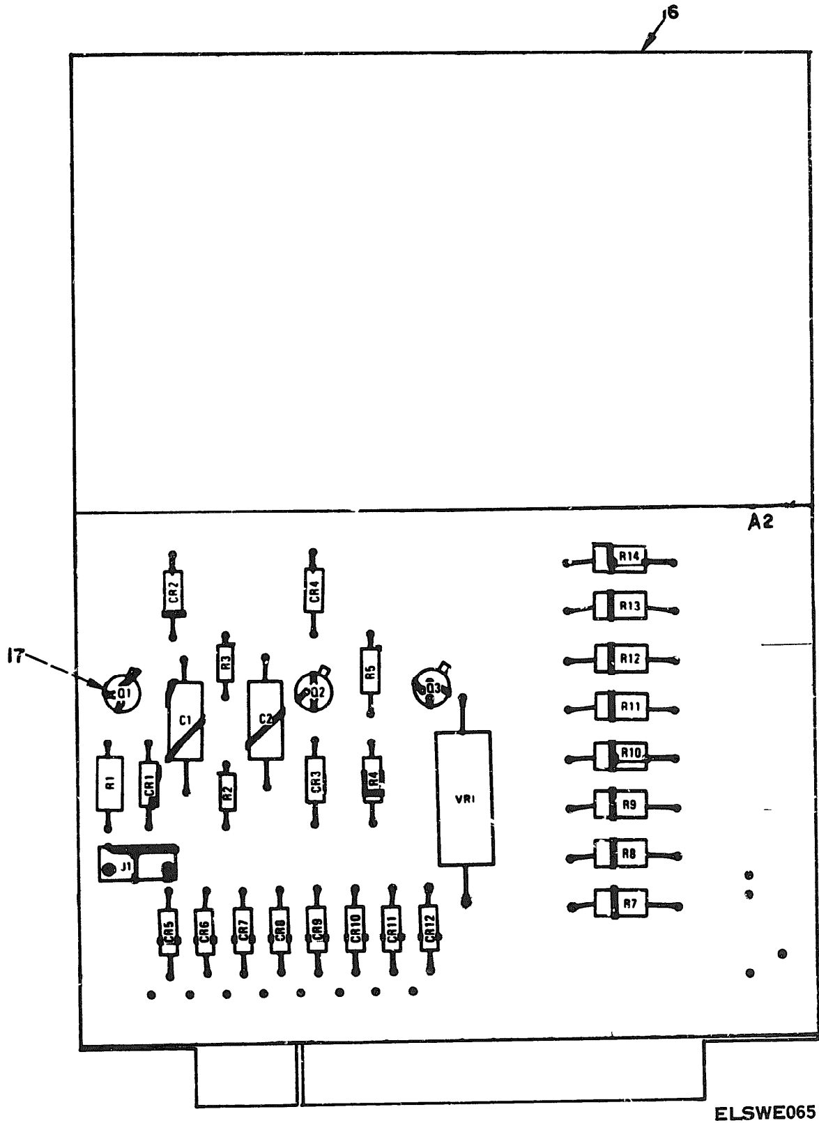
Figure 35. Offset Control Module 2A7 (Sheet 1 of 2)
