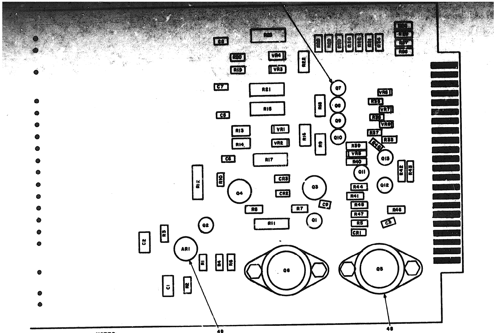
Figure 23. Yoke Simulator Module 2A1 (Sheet 1 of 2).
