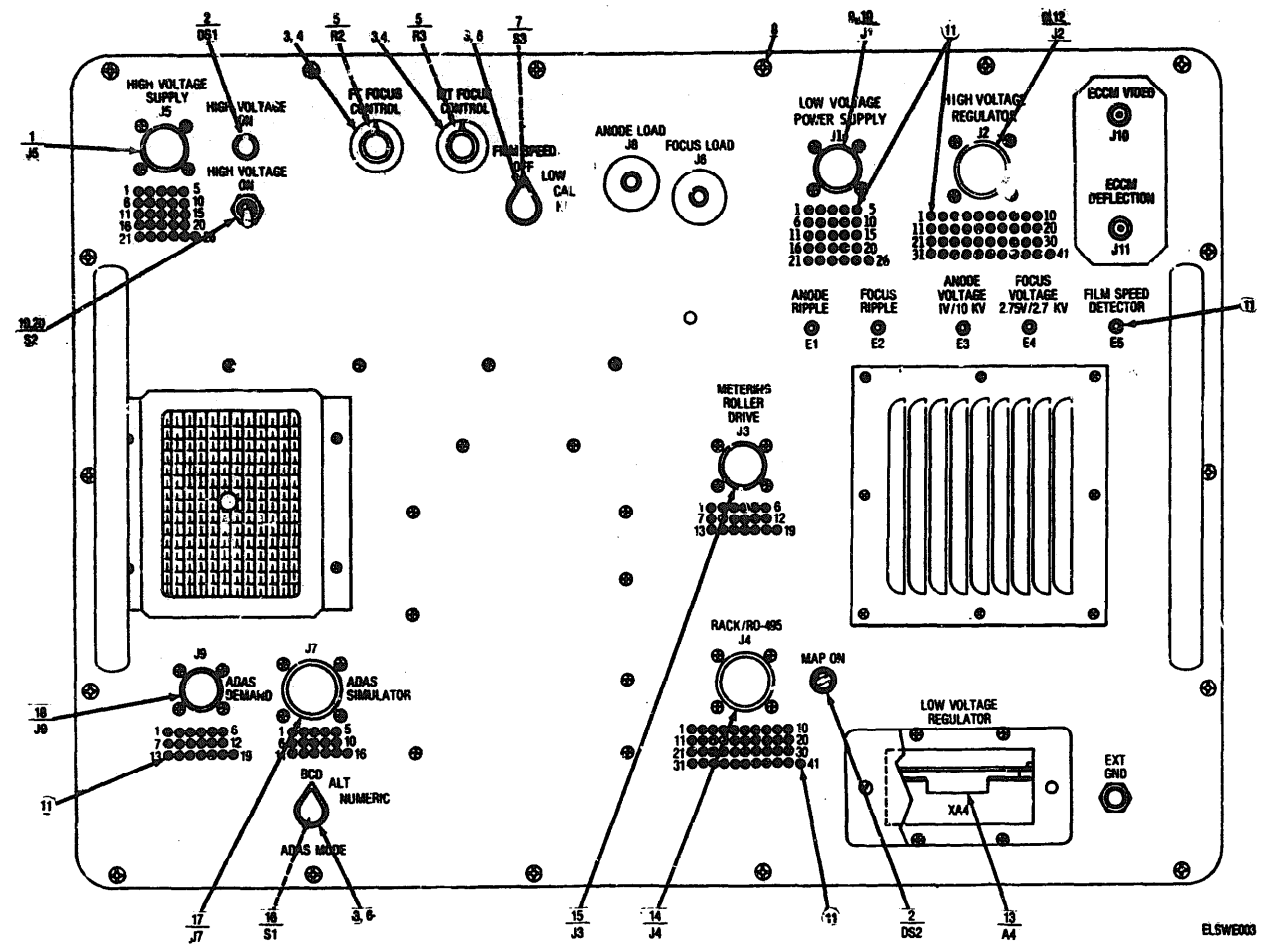
Figure 3. Electrical Test Panel 1A1 (Sheet 1 of 3).
